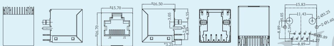
Recommended Pcb Layout Viewed From Component Side
