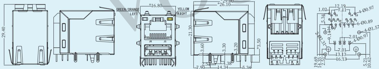
Recommended Pcb Layout Viewed From Component Side
