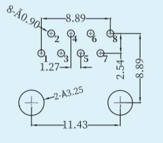
Recommended Pcb Layout Viewed From Component Side
