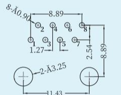
Recommended Pcb Layout Viewed From Component Side
