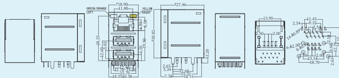
Recommended Pcb Layout Viewed From Component Side
