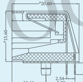
Cutaway View
