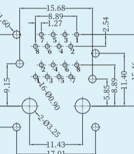
Recommended Pcb Layout Viewed From Component Side
