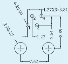
Recommended Pcb Layout Viewed From Component Side
