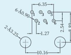
Recommended Pcb Layout Viewed From Component Side
