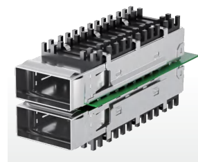
● Belly to Belly
